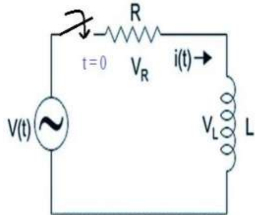
Figure3.1: RLCircuit
