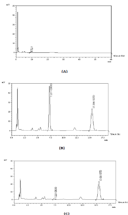
Fig. 2: Chromatograms of (A) blank human plasma; (B) human plasma sample spiked with 35 µg/mL of Levetiracetam and IS (HQC); (C) spiked human plasma sample at LLOQ (1 µg/mL). Approximate retention times: Levetiracetam = 7.2 min; IS = 15.4 min.
