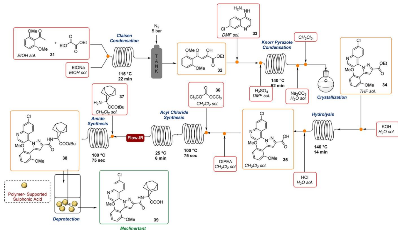
Scheme 6. Continuous Flow Synthesis of Meclintertant
