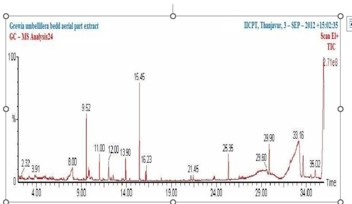
Fig. 1: GC-MS analysis of ethanolic GU aerial plant extract, The chromatogram showing n - Hexadecanoic Acid (53.91), 1,3-Propanediol, 2-(hydroxymethyl)-2-nitro-(8.24), Phytol (6.92) and \zeta -Sitosterol (4.17) peaks detected by GC-MS
